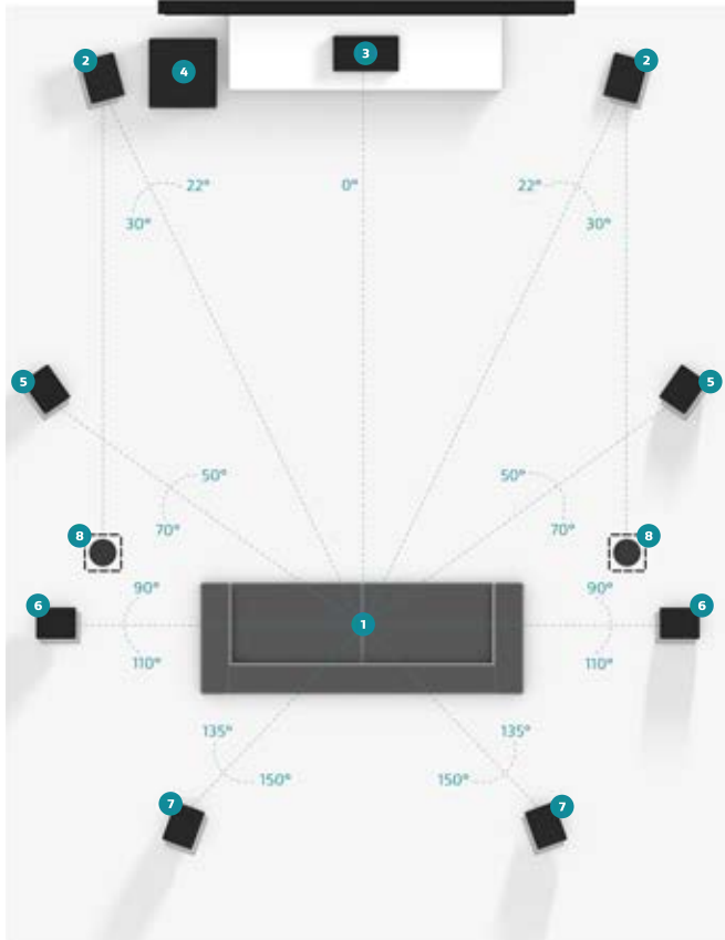
9.1.2 Speaker Placement
