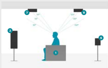
7.1.4 Ceiling Speaker Placement Detail
