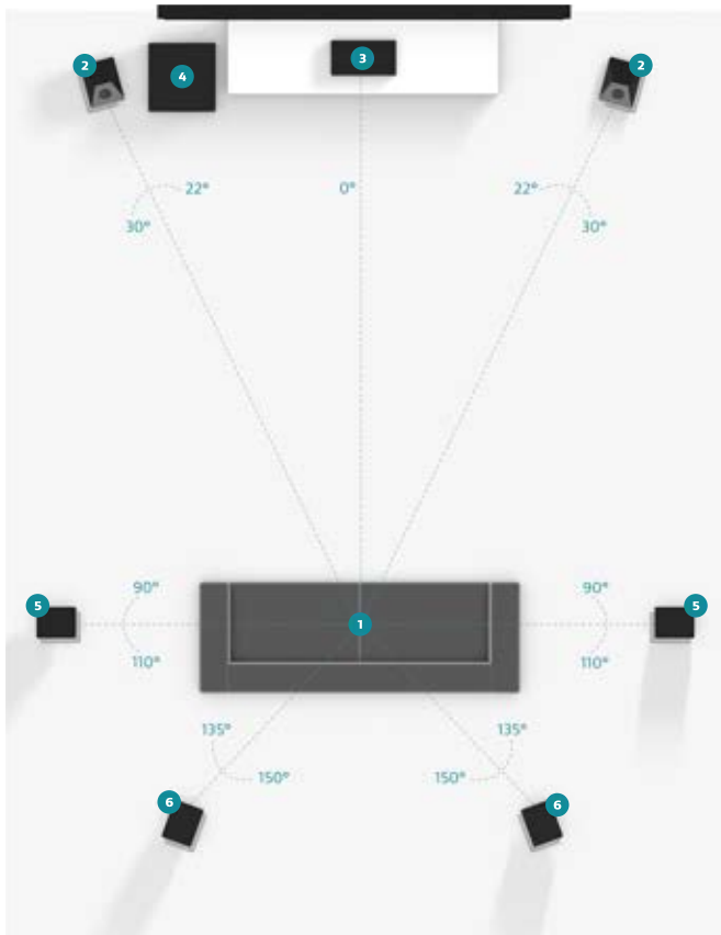
7.1.2 Speaker Placement
