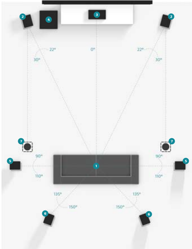
7.1.2 Speaker Placement
