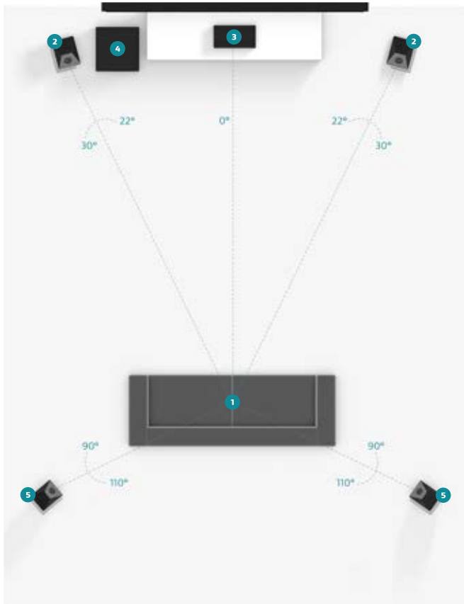
5.1.4 Speaker Placement
