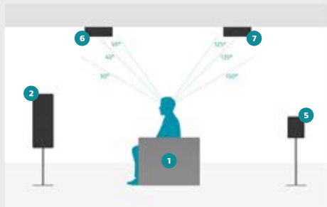
5.1.4 Ceiling Speaker Placement Detail
