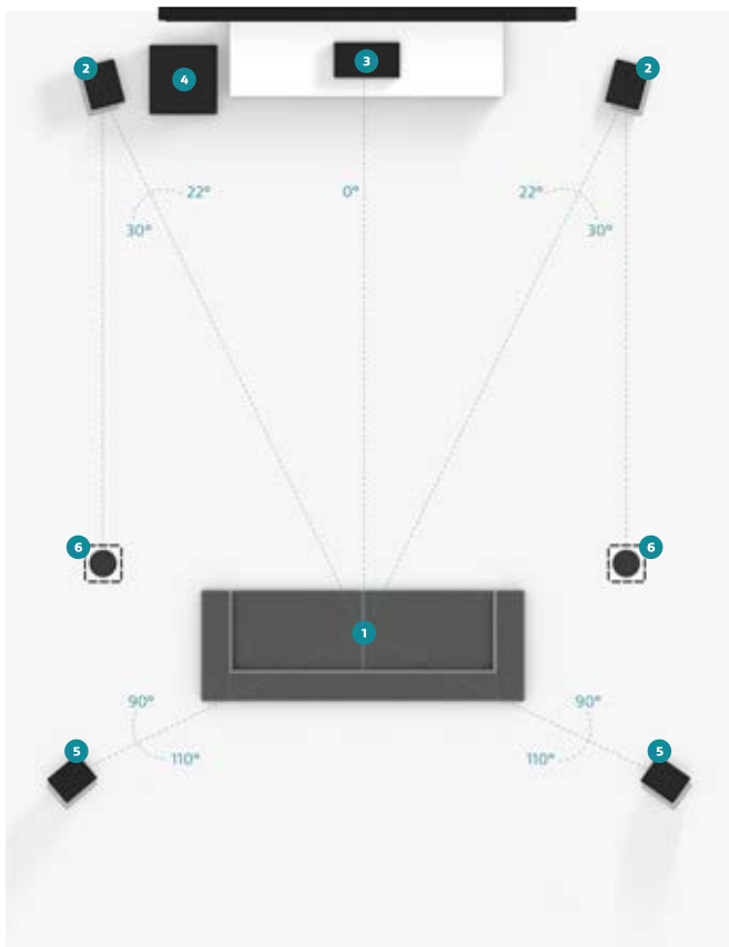
5.1.2 Speaker Placement
