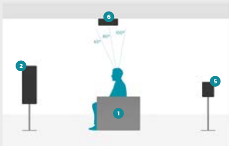
5.1.2 Ceiling Speaker Placement Detail
